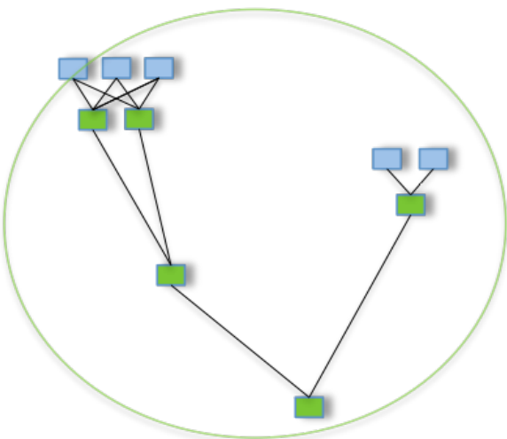
Pig/Hive - Tez
