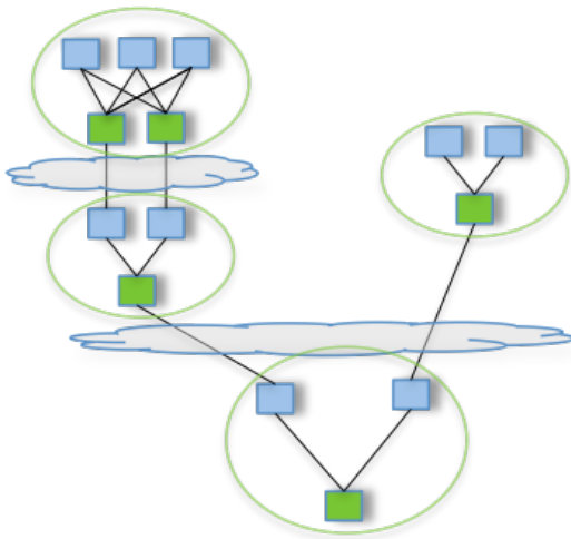
Pig/Hive - MR
